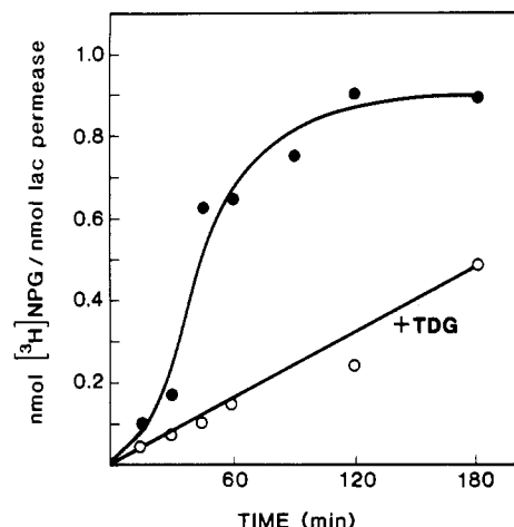
FIGURE 6: [^3\text{H}]\text{NPG} photoaffinity labeling of H322R membrane vesicles. RSO vesicles were resuspended to 1.5 mg of protein/mL in 0.1 M potassium phosphate (pH 6.6) and preequilibrated with an argon atmosphere in the presence of 20 mM lithium D-lactate (Kaczorowski et al., 1980). [^3\text{H}]\text{NPG} (10 Ci/mmol) was added to a final concentration of 20 \mu\text{M} , and the sample was illuminated. At various times, 50- \mu\text{L} aliquots were removed and mixed with 3 mL of ice-cold 10% trichloroacetic acid. Precipitated protein was collected by filtration and assayed for radioactivity by liquid scintillation spectrometry. A parallel experiment was carried out in the presence of 20 mM TDG (○). Although data are not shown, after 60-min illumination in the absence of TDG essentially all of the radioactivity is associated with the 33-kDa band identified as lac permease [cf. Kaczorowski et al. (1980)].
